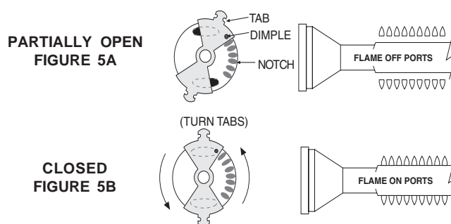
Figure 5A & 5B - Air Shutter Adjustment Diagram
