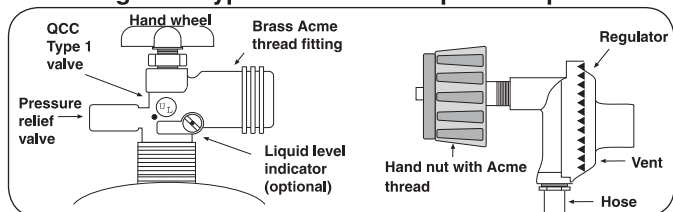
Fig. 11-1 Type I Acme thread quick coupler
