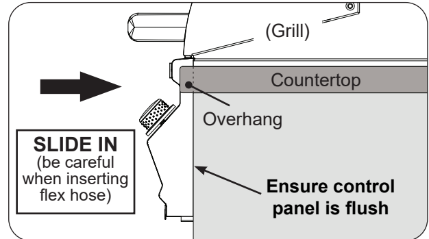
Fig. 24-2 Slide in unit (ensure flush)
