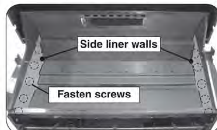
Fig. 2-4 Install side liner walls
