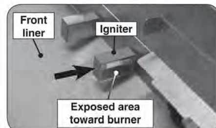
Fig. 2-6 Install igniters
