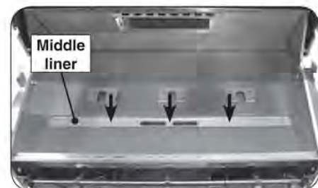
Fig. 1-3 Install middle liner
