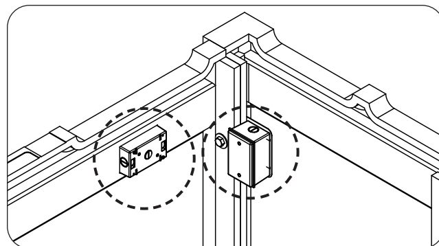
Fig. 8-4 Install electrical (as needed)
