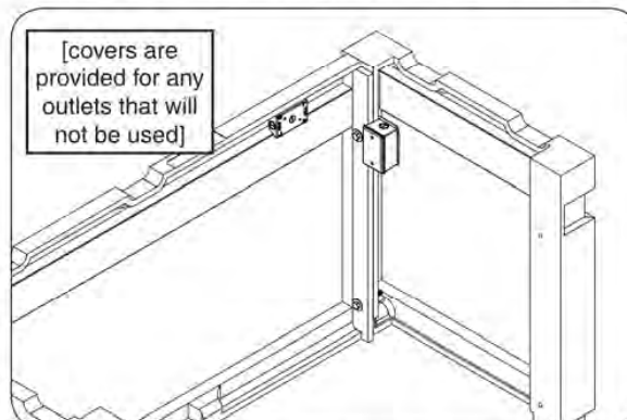
Fig. 7-4 Right wall and outlet box installed
