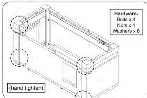
Fig. 8-1 Assemble front wall
