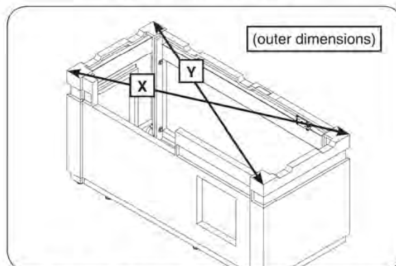
Fig. 8-3 Square unit (then tighten bolts)
