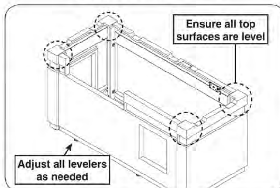
Fig. 8-2 Level assembly
