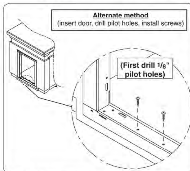
Fig. 9-3 Alternate door/drawer install method
