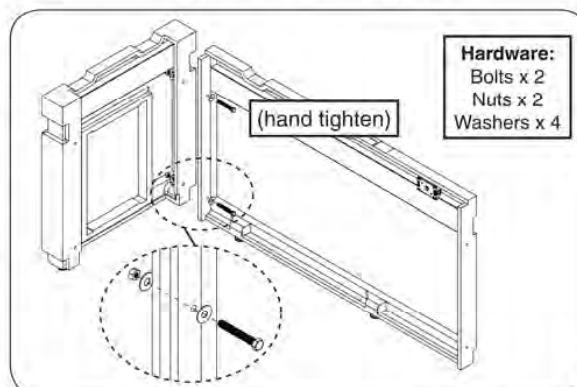
Fig. 7-2 Assemble rear and left wall
