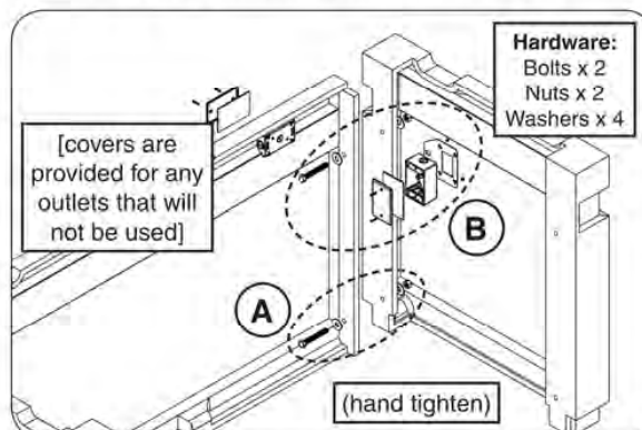
Fig. 7-3 Assemble right wall and outlet box
