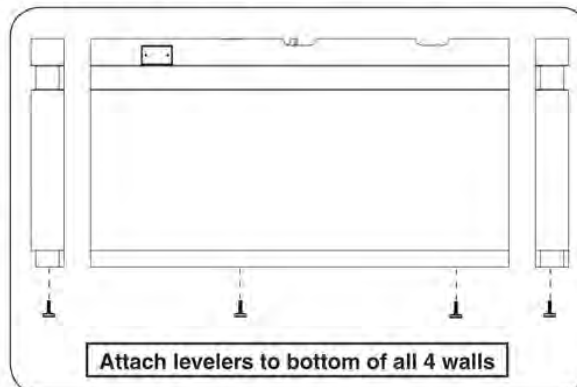
Fig. 7-1 Attach levelers
