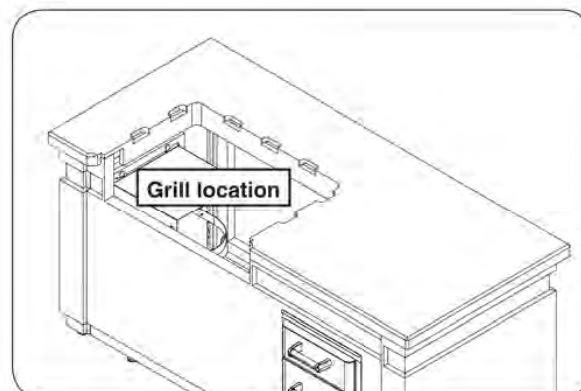
Fig. 11-3 Install grill
