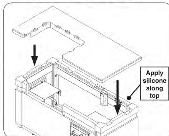
Fig. 11-2 Place countertop
