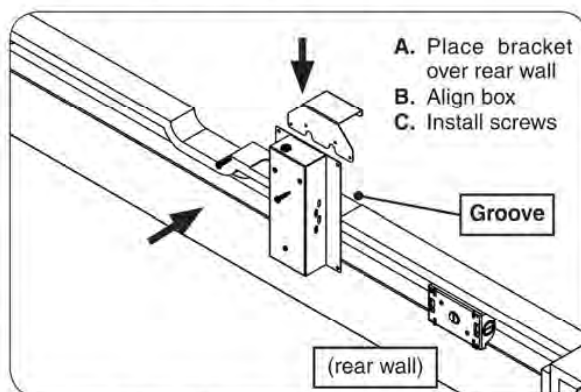
Fig. 11-1 Install power supply box
