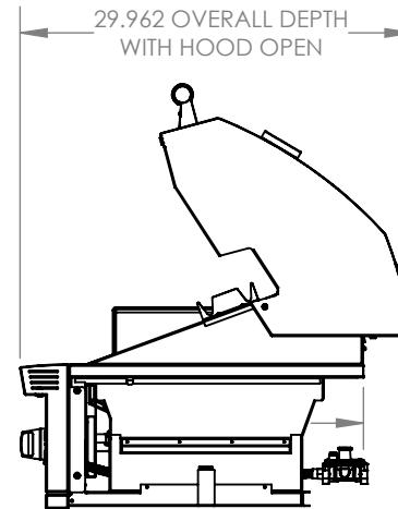
SIDE VIEW WITH HOOD OPEN
