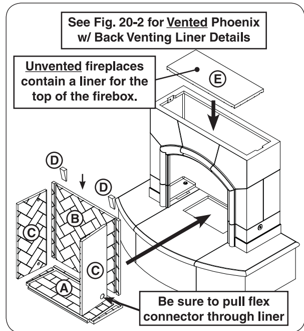
Fig. 20-1 Install firebox liners
