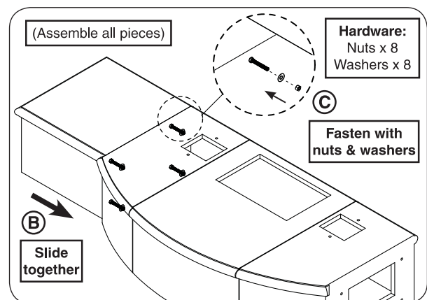
Fig. 17-2 Assemble hearth - slide together & fasten
