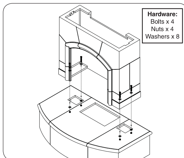
Fig. 18-1 Assemble body
