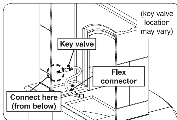
Fig. 18-3 Route gas supply (underneath install)
