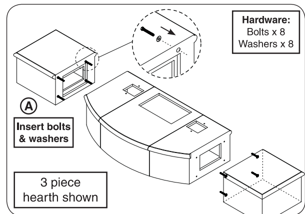
Fig. 17-1 Assemble hearth - arrange (if required)
