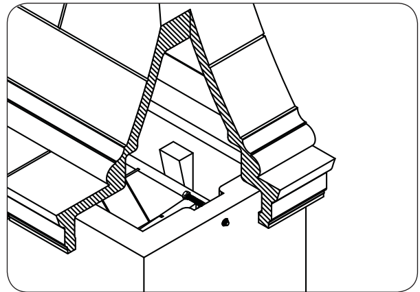
Fig. 21-2 Bolt detail
