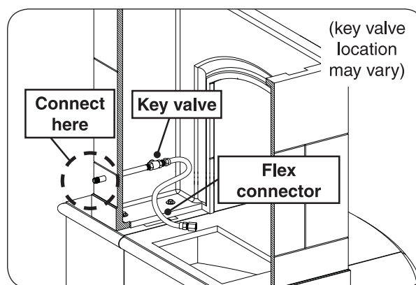
Fig. 18-2 Route gas supply (rear install)
