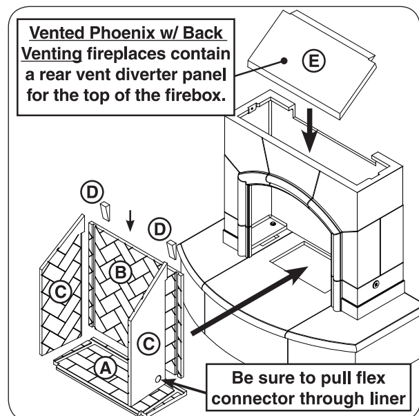
Fig. 20-2 Install liners ( Vented Phoenix w/ Back Venting)
