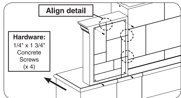
Fig. 19-2 Assemble rear side-wall (skip if n/a)
