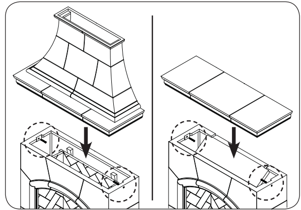
Fig. 21-1 Assemble chimney / mantel
