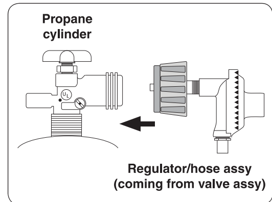
Fig. 17-1 Connecting to an L.P. cylinder
