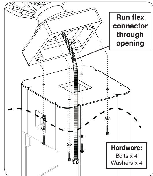
Fig. 16-1 Place urn and secure
