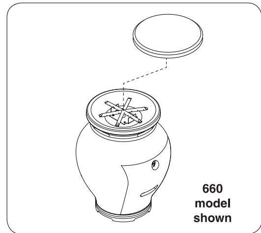
Fig. 20-1 GFRC cover placement
