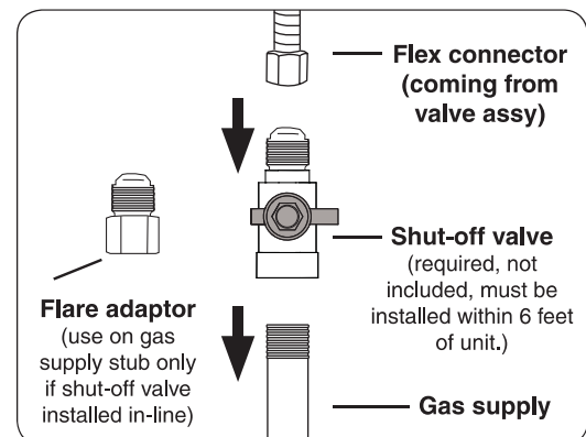
Fig. 17-3 Connecting to a gas line
