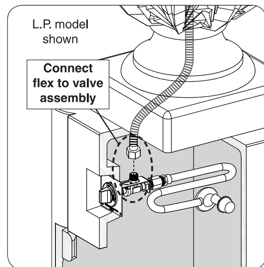
Fig. 16-2 Connect flex to valve
