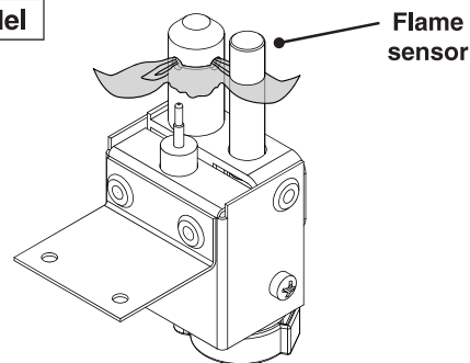
Fig. 31-2 Proper pilot flame
