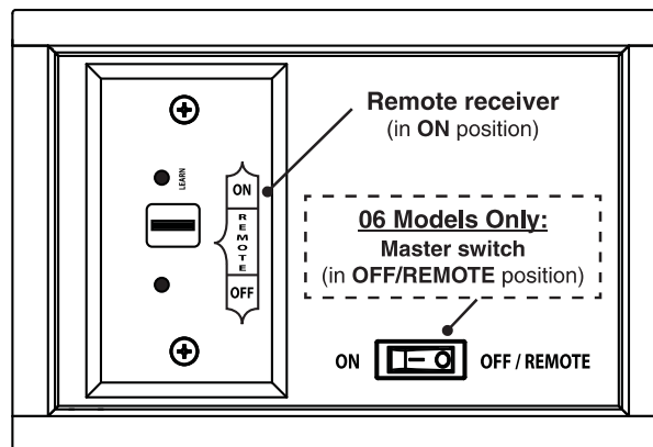
Fig. 31-1 Control panel detail
