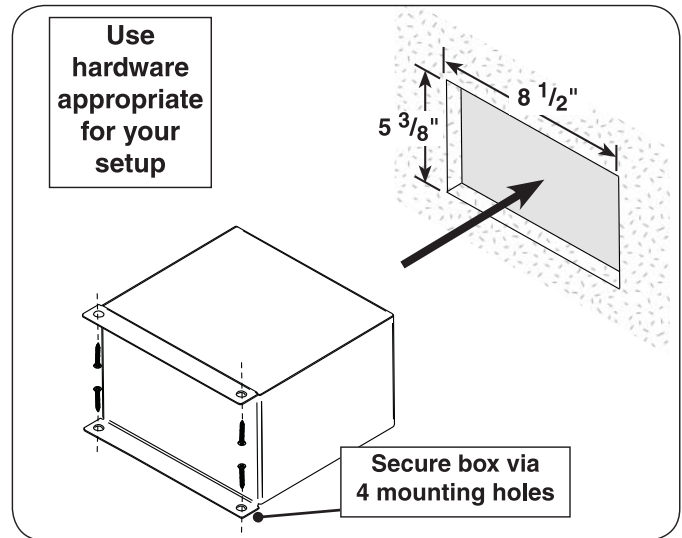
Fig. 22-1 Install control box (if applicable)
