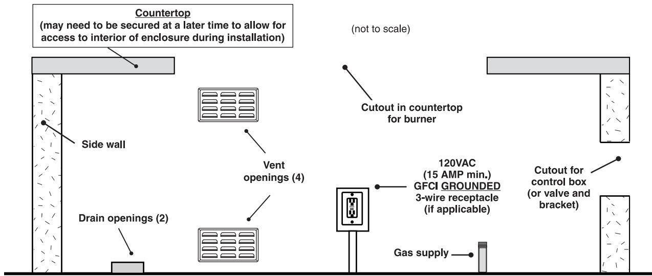
Fig. 21-1 Enclosure construction overview (side view)
