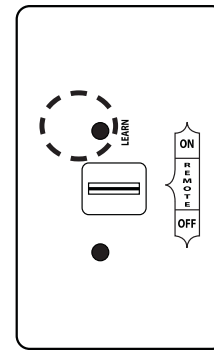
Fig. 34-1 Remote receiver sync detail
