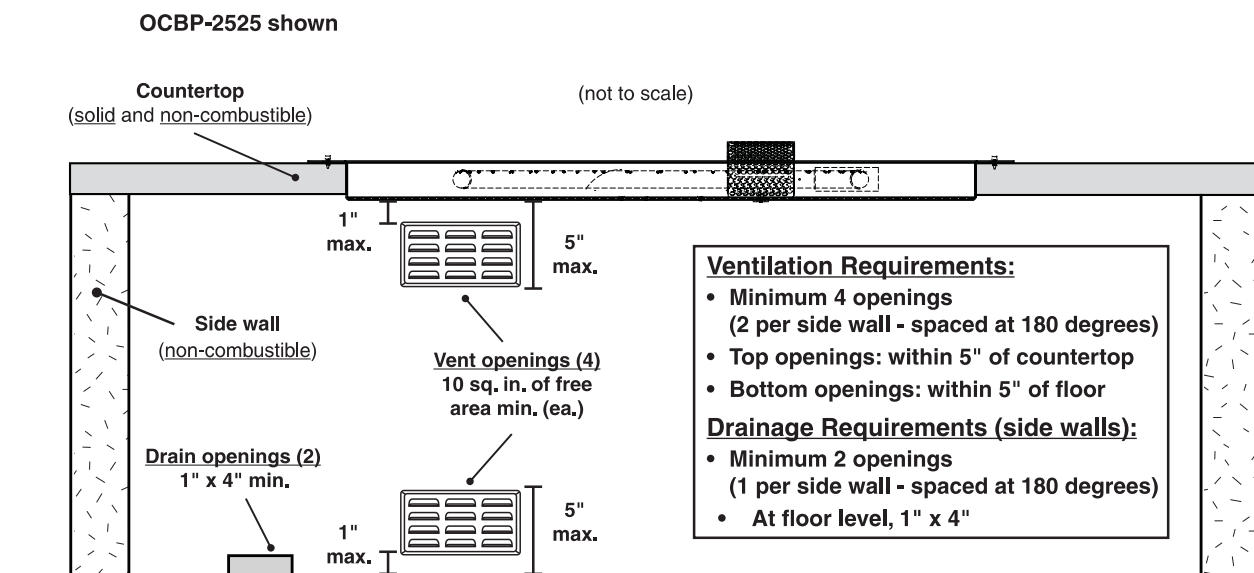
Fig. 13-2 Ventilation and drainage specifications (enclosure side view)
