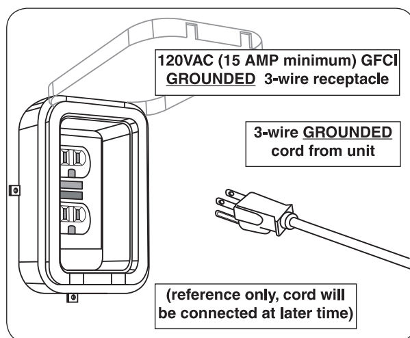
Fig. 20-2 Electrical setup detail
