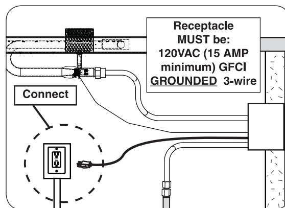
Fig. 23-1 Route and connect power supply cord
