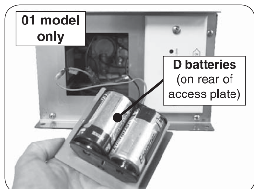
Fig. 35-5 Burner system batteries
