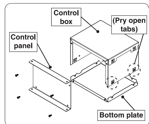
Fig. 42-4 Control panel interior access
