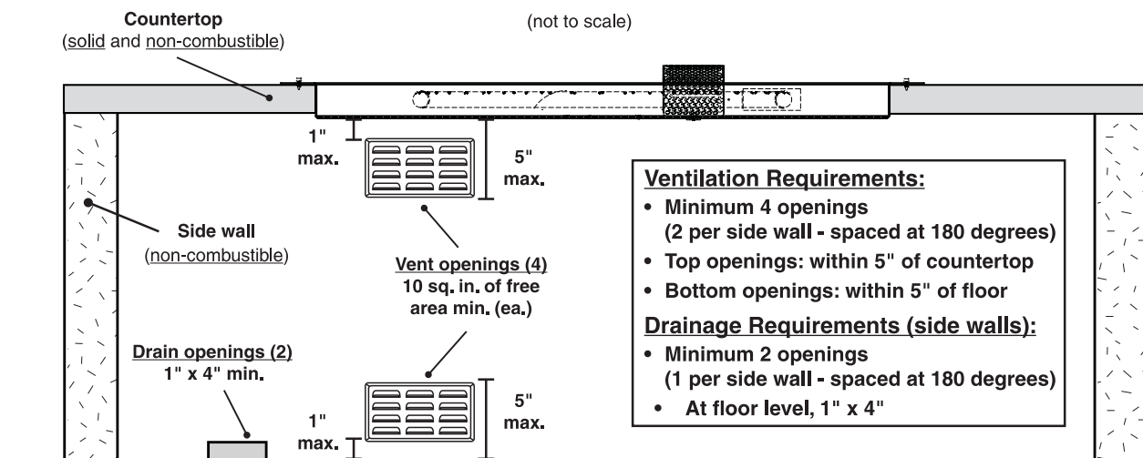
Fig. 13-2 Ventilation and drainage specifications (enclosure side view)
