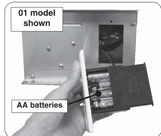
Fig. 43-4 Remote receiver batteries
