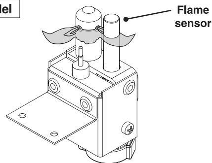
Fig. 39-2 Proper pilot flame
