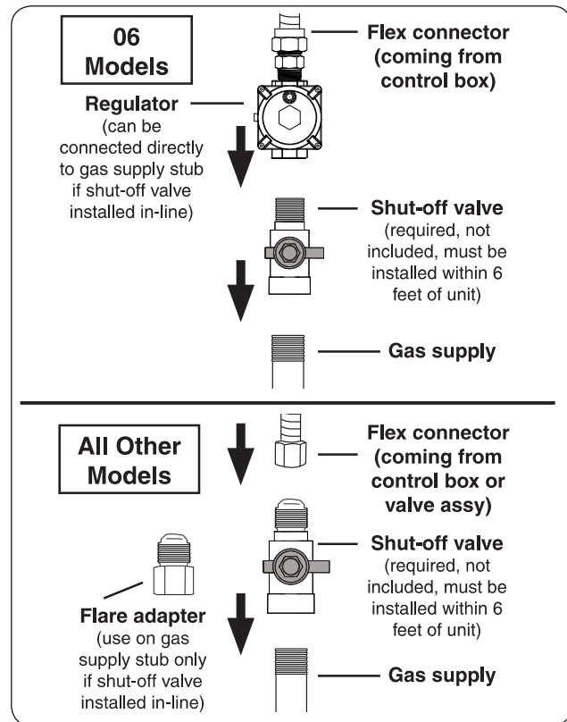
Fig. 25-1 Connecting to a gas line
