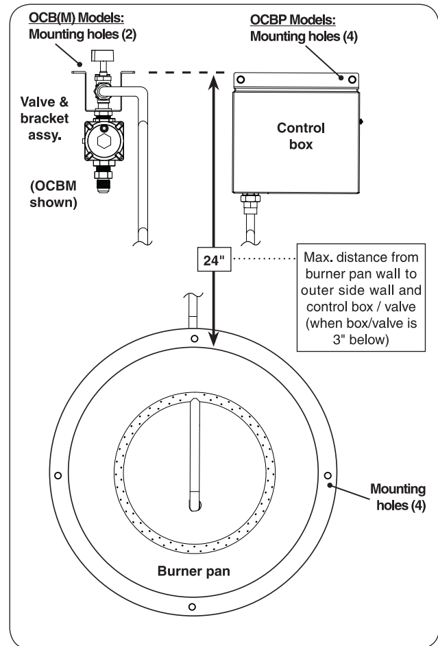
Fig. 12-1 Mounting detail (top view)
