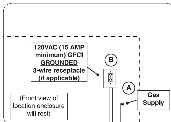
Fig. 22-1 Route gas and electrical (receptacle)
