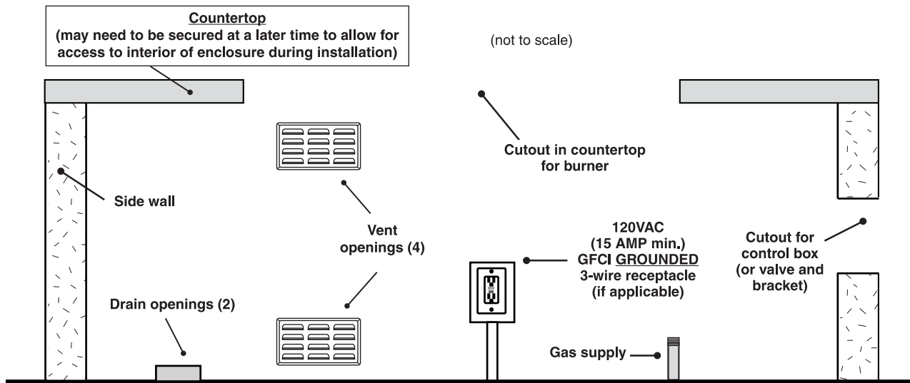
Fig. 23-1 Enclosure construction overview (side view)
