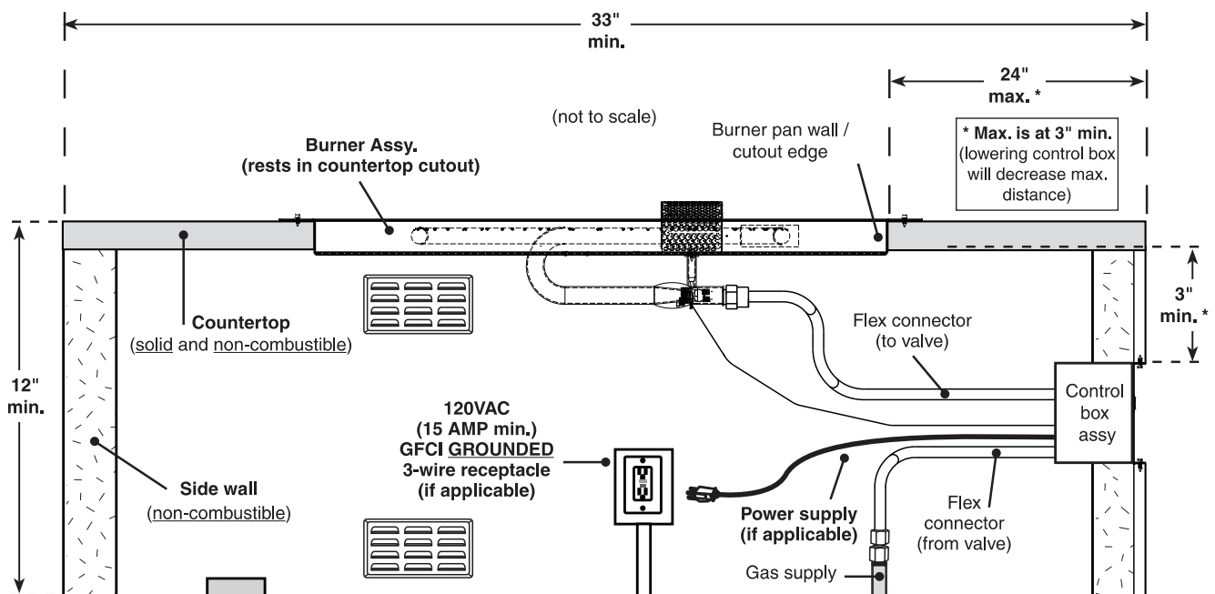
Fig. 11-2 Enclosure specifications (side view)
