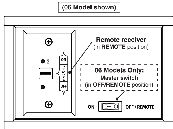
Fig. 37-1 Control panel detail
