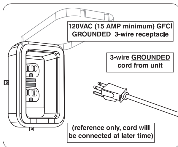
Fig. 22-2 Electrical setup detail
