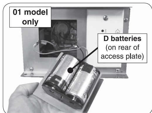
Fig. 43-5 Burner system batteries
