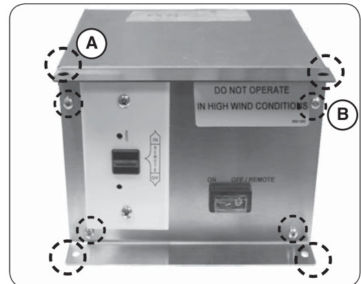
Fig. 42-2 Remove screws to access fuse
