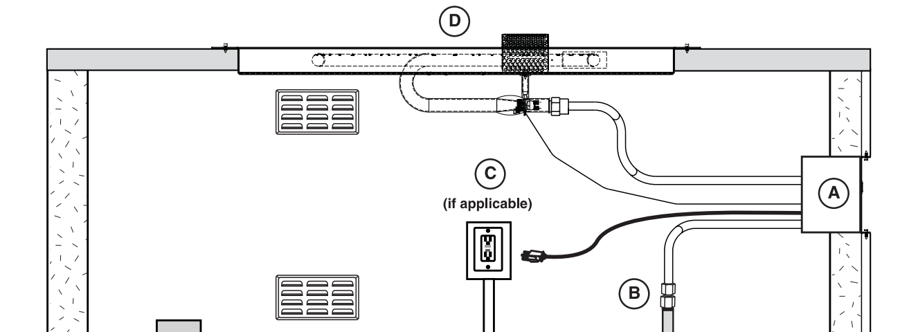
Fig. 23-2 Install burner system
