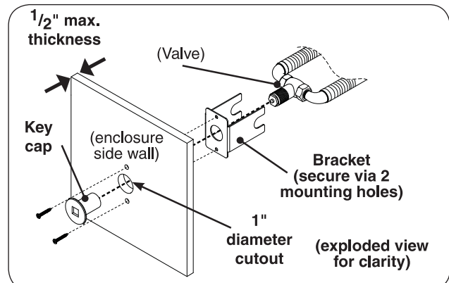
Fig. 24-3 Install valve & bracket assy (if applicable)
