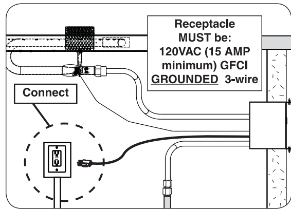
Fig. 26-1 Route and connect power supply cord
