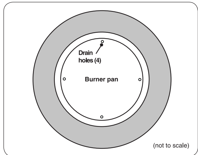
Fig. 13-1 Burner pan drainage (top view)
