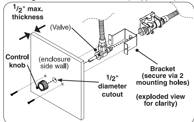
Fig. 24-2 Install valve & bracket assy (if applicable)
