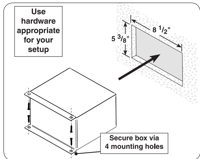
Fig. 24-1 Install control box (if applicable)
