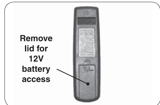
Fig. 43-3 Transmitter battery
