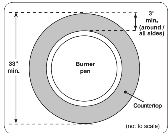
Fig. 11-1 Countertop minimum (top view)
