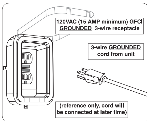
Fig. 21-2 Electrical setup detail
