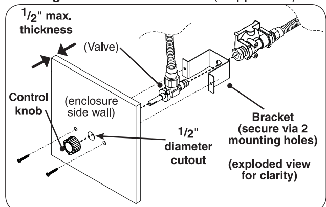
Fig. 23-2 Install valve & bracket assy (if applicable)
