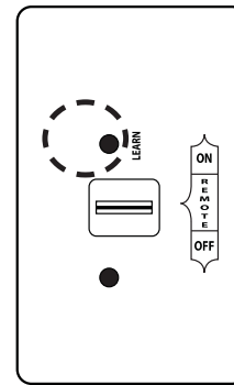
Fig. 40-1 Remote receiver sync detail
