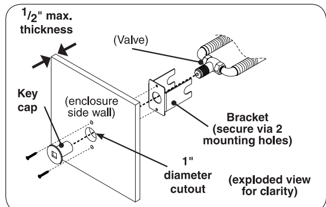
Fig. 23-3 Install valve & bracket assy (if applicable)
