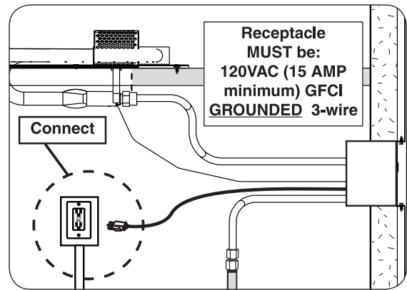
Fig. 25-1 Route and connect power supply cord
