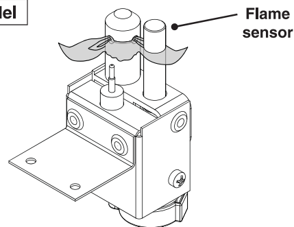
Fig. 37-2 Proper pilot flame
