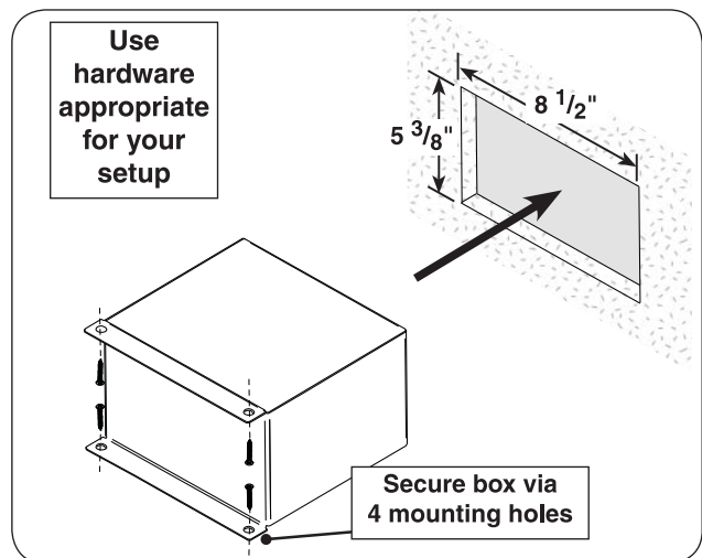
Fig. 23-1 Install control box (if applicable)
